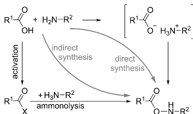
Fig. 1. General scheme of amide synthesis, adopted from refs [24,27].
