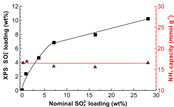
Fig. 12. SO 4 2- surface loading (left y-axis) and total NH 3 chemisorption capacity (right y-axis) as a function of nominal composition in the T1S catalysts.
