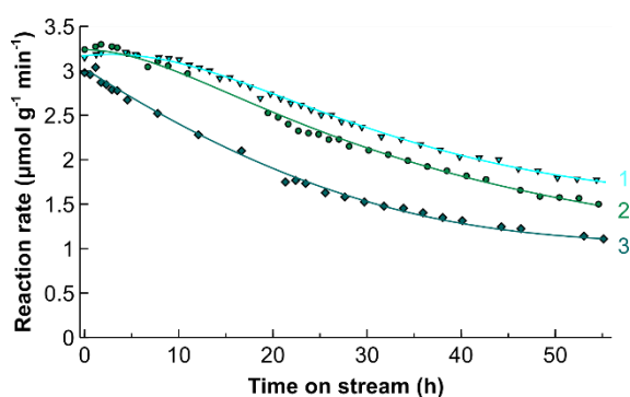
Fig. 16. Reaction rate as a function of time on stream catalysed by the T3S1 catalyst over 2 regeneration cycles with H 2 O 2 . Reaction conditions: flow rate of 40 µL min -1 (50 mM 4-phenylbutyric acid, 50 mM aniline), 320 mg of the catalyst, 150 °C, 7 bar(g) in the RF-heated reactor.
