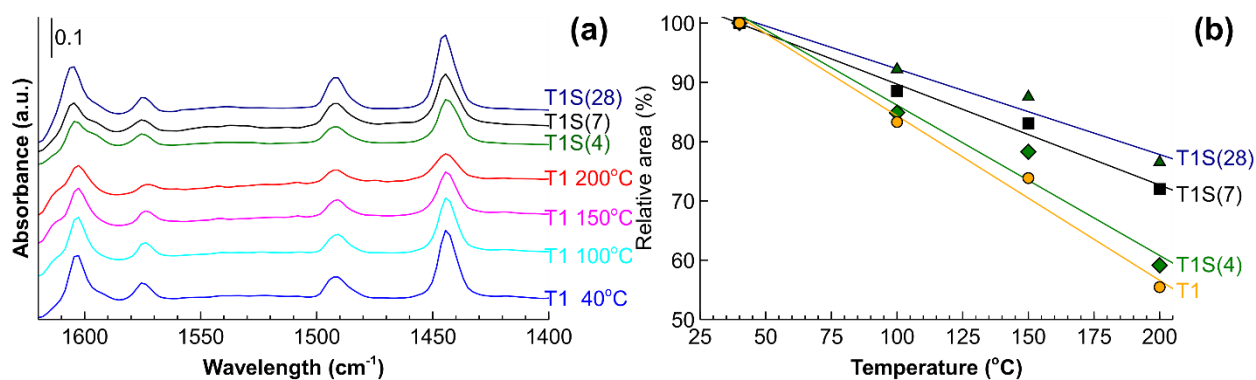
Fig. 13. (a) FTIR spectra of pyridine over sulfated titania catalysts and (b) temperature dependence of normalised intensity of the 1445\text{ cm}^{-1} band at 40\text{ }^{\circ}\text{C} .
