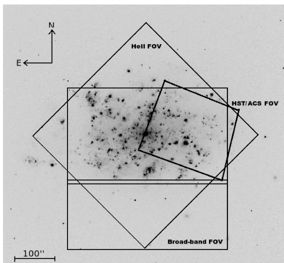
Figure 1. CTIO wide-field H\alpha image of NGC 7793 (Kennicutt et al. 2008), showing the field of view (FOV) of the B, V, H\alpha images (‘broad-band’), archival \text{He II} & [\text{O III}] images, and the HST/ACS F555W images.
