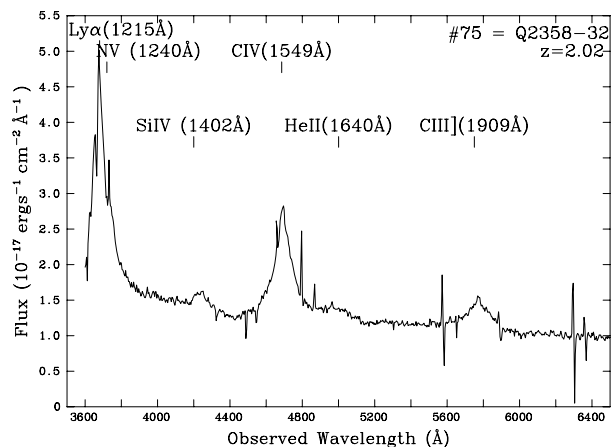
Figure 12. FORS1 spectrum of the background quasar Q2358-32 which lies at z = 2.02 . This source was picked up in our WR survey because \text{C IV } \lambda 1548-51 was redshifted into the \lambda_c = 4684 \text{ \AA} narrow-band filter.
