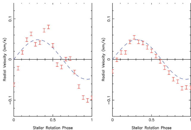
Figure 11. Left-hand panel: RV curve of the G5V model star with four dark spots ( T_{\text{spot}} = 4600 K) each covering 1 per cent of the visible surface at positions (detailed in Table 1) and a 1 Jupiter mass planet on a 4 d orbit. Right-hand panel: RV curve after 21 iterations of the spot removal code.
