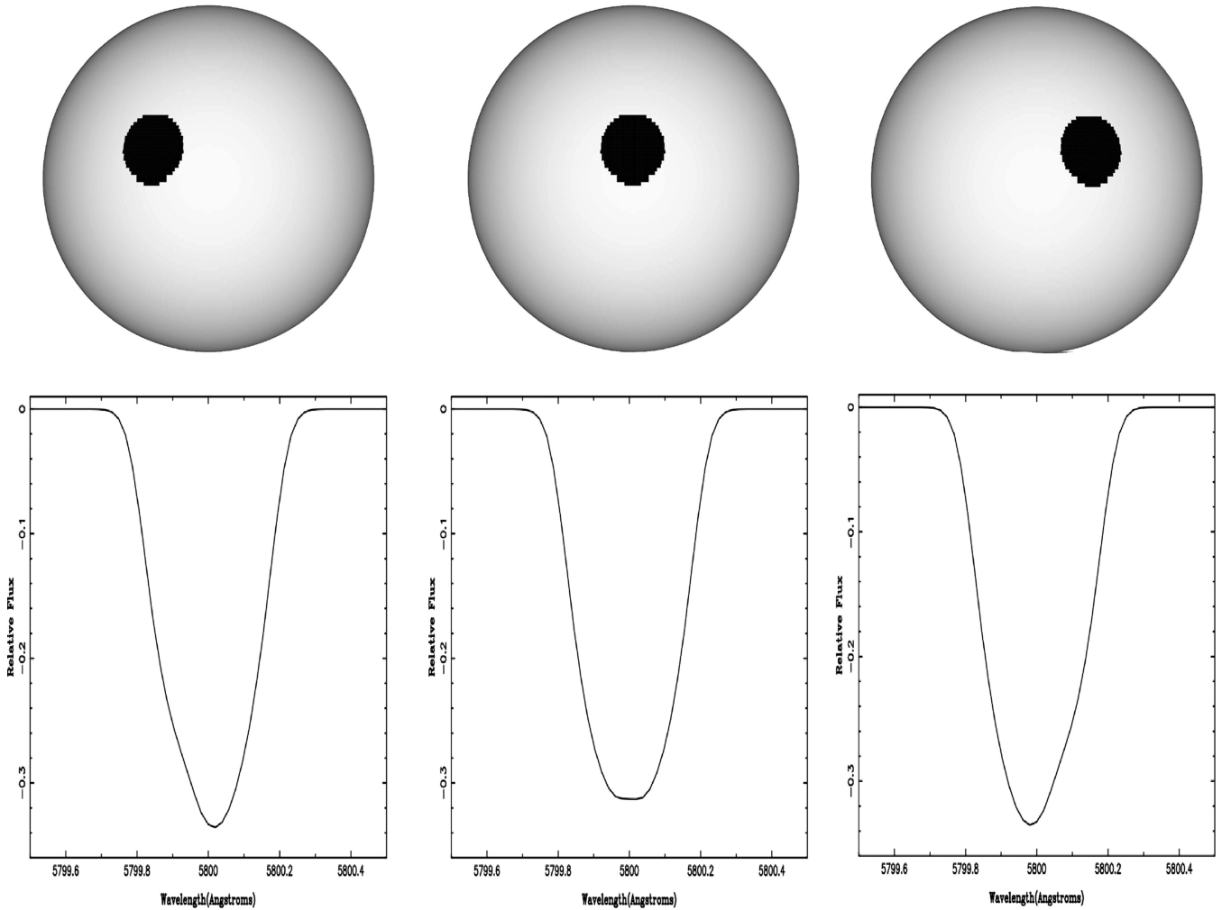
Figure 2. The effect of a rotating star spot on the rotationally broadened line-profile. The top panels show the model star at different phases while the lower panel represents the line-profiles at this corresponding phase.
