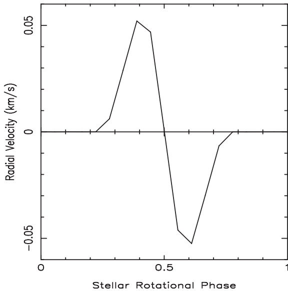
Figure 4. The RV for a G2V type star seen face on with a dark spot ( T_{\text{spot}} = 0\text{ K} ) covering 1.05 per cent of the visible surface at \theta = 0^\circ .
