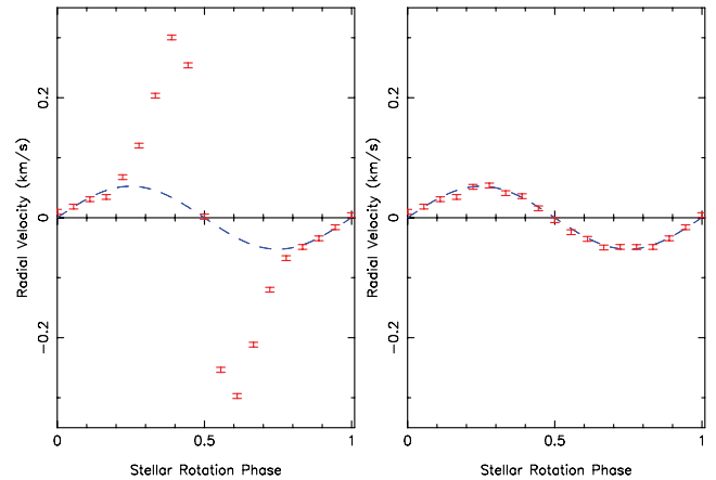
Figure 9. Left-hand panel: RV curve of the G5V model star with a dark spot ( T_{\text{spot}} = 4600 K) covering 5 per cent of the visible surface at a latitude of 20^\circ and a 1M_J planet on a 3.2 d orbit. Right-hand panel: RV curve after the spot removal code is applied to the data. As can be seen CLEARASIL is successful at reducing the RV noise to reveal a periodic signal that closely matches the signal of the injected planet.
