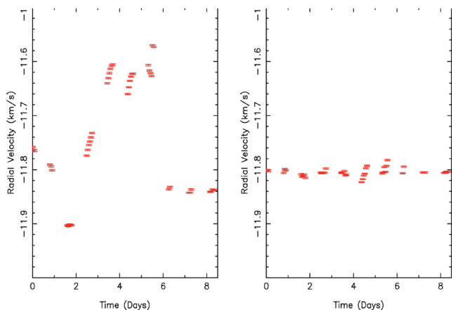
Figure 15. Left-hand panel: RV curve of HD 49933. Right-hand panel: RV curve after the spot removal code.
