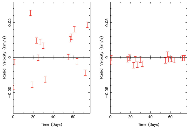
Figure 12. Left-hand panel: RV curve of the G5V model star with random spot coverage ( T_{\text{spot}} = 4600 K) with positions and sizes detailed in Table 2. Right-hand panel: RV curve after 18 iterations of the spot removal code.
