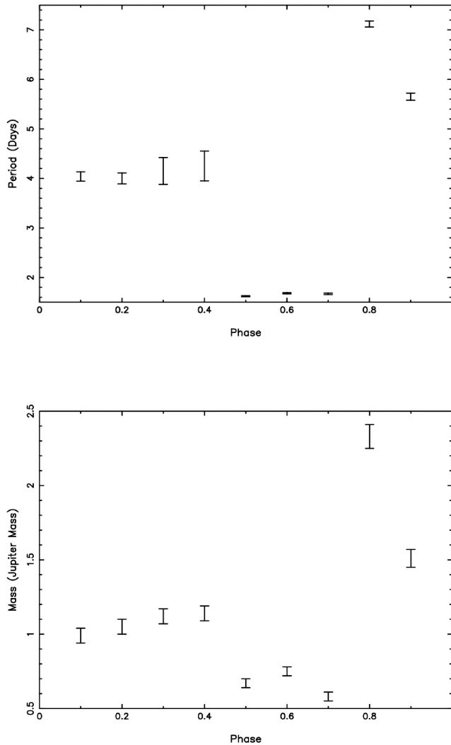
Figure 8. Results showing the impact of varying the planet signal phase on the ability of CLEARASIL to uncover the correct planet signature. In this case a G5V model star with a dark spot ( T_{\text{spot}} = 4600 K) covering 5 per cent of the visible surface at a latitude of 20^\circ and a 1M_J planet on a 4 d orbit was used. The phase of the planet was varied from 0 to 1 in steps of 0.1. The top panel displays how the planetary period uncovered by CLEARASIL varies with the injected planetary phase, while the bottom panel shows the planetary phase against the mass of the uncovered planet signal.
