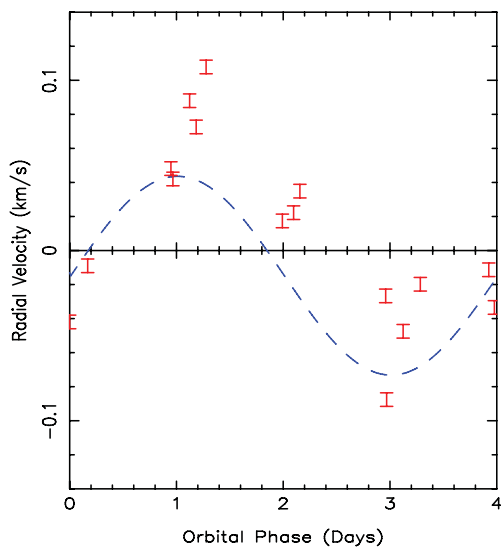
Figure 13. RV curve of the G5V model star with random spot coverage (spot parameters are detailed in Table 2) and a 1 Jupiter mass planet on a 4d orbit. Overplotted on this curve is a blue dashed line showing the best sine fit to these ‘noisy’ data.
