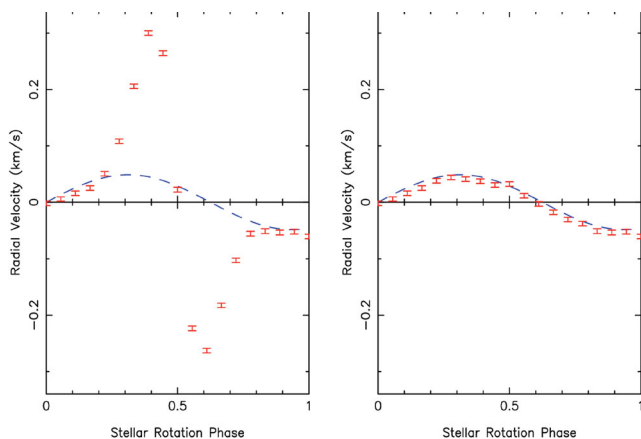
Figure 7. RV results for the G5V model star which has both a dark spot ( T_{\text{spot}} = 4600 K) covering 5 per cent of the visible surface at a latitude of 20^\circ and a 1 M_J planet on a 4 d orbit. The red bars represent the RV points of the model data, while the blue dashed line corresponds to the RV of the 1 M_J planet that has been injected into the model. The RV of the simulated observational line-profiles is shown in the left panel, while the right panel shows the RVs after using CLEARASIL to remove any spot features present. As can be seen, the injected planet signature is well recovered from the noise.
