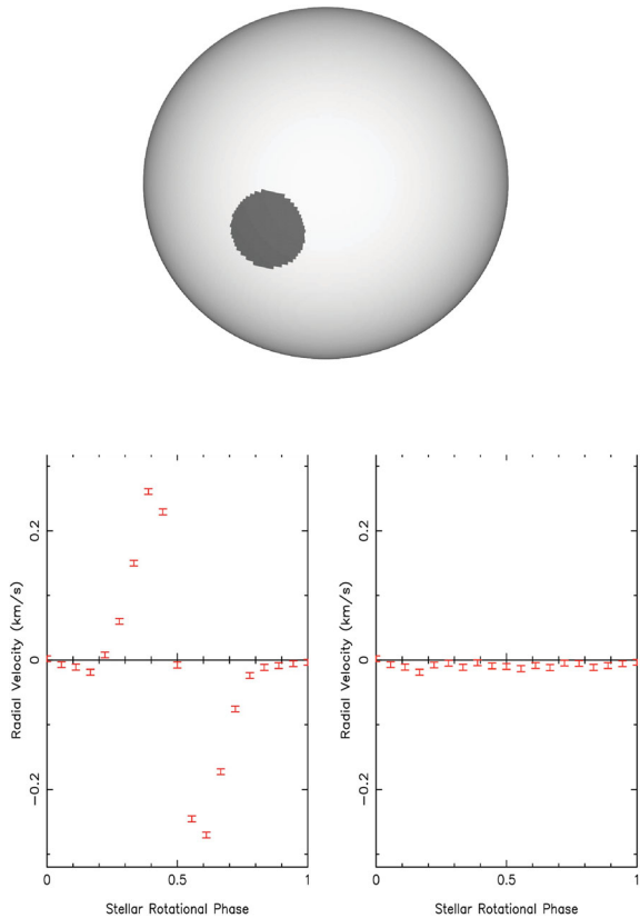
Figure 6. Top: the model G5V star with dark spot ( T_{\text{spot}} = 4600 K) covering 5 per cent of the visible surface at a latitude of 20^\circ . Bottom left panel: the RV points determined using the 19 model line-profiles that were generated for this one-spot star. Bottom right panel: the RV results after using CLEARASIL to clean spots from the model data. The RV jitter due to the spot is reduced by 98 per cent in this test.
