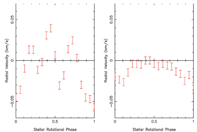
Figure 10. Left-hand panel: RV curve of the G5V model star with four dark spots ( T_{\text{spot}} = 4600 K) each covering 1 per cent of the visible surface at positions detailed in Table 1. Right-hand panel: RV curve after 13 iterations of the spot removal code. As can be seen CLEARASIL is successful at reducing the RV noise by 75 per cent.
