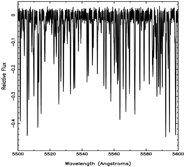
Figure 3. Example portion of a synthetic spectrum generated by our model, assuming a G5V type star ( M_* = 1.05M_{\text{sun}} , R_* = 0.95R_{\text{sun}} , T_{\text{eff}} = 5657\text{ K} , P_{\text{rot}} = 3.2\text{ d} and i = 51.8^\circ ) with a 5 per cent spot having a peak SNR of 100 and a v \sin i = 15\text{ km s}^{-1} .
