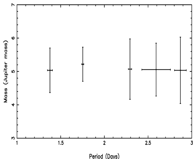
Figure 16. The mass of a planet as a function of the planetary period when using CLEARASIL to uncover approximately five Jupiter mass planets injected into the HD 49933 data. The error bars represent the difference between the fitted and the simulated parameters.
