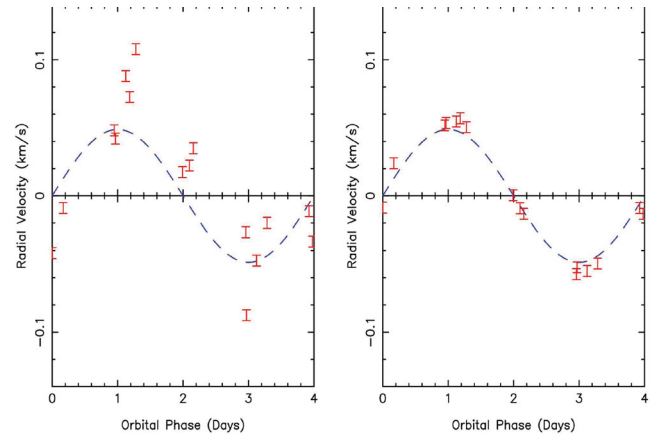
Figure 14. Left: RV curve of the G5V model star with random spot coverage (spot parameters are detailed in Table 2) and a 1 Jupiter mass planet on a 4 d orbit. Right: RV curve after nine iterations of the spot removal code. In both plots, the data have been phase folded on to the orbital period of the fake planet injected into the data.
