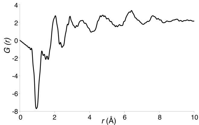
FIG. 2. Neutron-diffraction generated all-ion PDF for fully-hydrated synthesized 2-line ferrihydrite. The large negative trough at 0.95 Å is accounted for by an O-H correlation.
