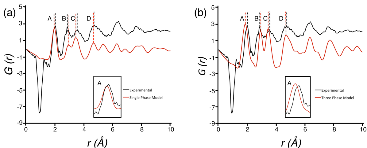
FIG. 3. Neutron-diffraction generated all-ion PDF for synthetic 2-line ferrihydrite (black) compared with, in red, (a) the all-ion PDF of the original single-phase 2-line model [15] and (b) the 3-phase model [10]. The fully crystalline model PDFs have been attenuated using an exponential function, G(r) = G(r)_0 \cdot e^{-0.234r} , to mimic the decay signal at larger distances ( r -values) that would be found in a nanoparticulate sample. This exponential was intended not as a fit to the experimental data, but simply to remove the long-range crystallinity inherent in the modelled PDFs. The insets show Peak A, which represents the first Fe-O bond length, in detail.
