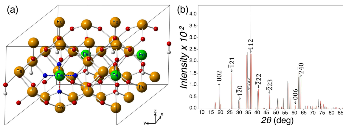
FIG. 5. (a) DFT-optimized single-phase 2-L ferrihydrite. The tetrahedral Fe ions are shown in green and the octahedral Fe ions in orange. In this new structure, the tetrahedral Fe site is reduced by 17 % compared to the original single-phase model [15]. The new Fe tet -O bond lengths are 1.883 Å (blue-banded) and 1.864 Å (red-banded). The directly bonded oxygen atoms for the example tetrahedral sites are shown in dark blue, all other oxygen ions are shown in red and hydrogen in white. For clarity some ions have been removed from the illustration to make the example tetrahedral
