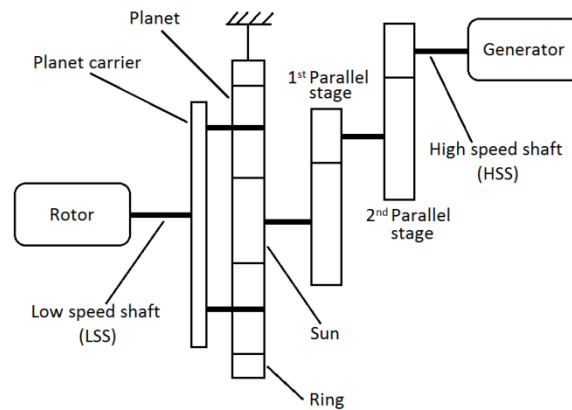
Figure 1. Simplified schematic of wind turbine drivetrain
