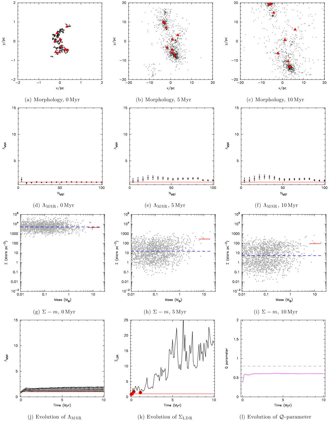
Figure 2. Evolution of a superviral ( \alpha_{\text{vir}} = 1.5 ), substructured star-forming region ( D = 1.6 ) with N = 1500 stars. We show the morphology at 0, 5 and 10 Myr (a–c), the mass segregation ratio, \Lambda_{\text{MSR}} of the N_{\text{MST}} most massive stars at 0, 5 and 10 Myr (d–f), and the surface density as a function of stellar mass, \Sigma - m (g–i) at 0, 5 and 10 Myr. We also show the evolution of \Lambda_{\text{MSR}} in panel (j) – the solid, dashed and dot–dashed lines are the values of \Lambda_{\text{MSR}} for the 10, 20 and 50 most massive stars, respectively; the ratio of the surface density of the 10 most massive stars to the median surface density of all stars in the region ( \Sigma_{\text{LDR}} = \bar{\Sigma}_{10}/\bar{\Sigma}_{\text{all}} – panel k) and the evolution of the Q -parameter (panel l), with time.
