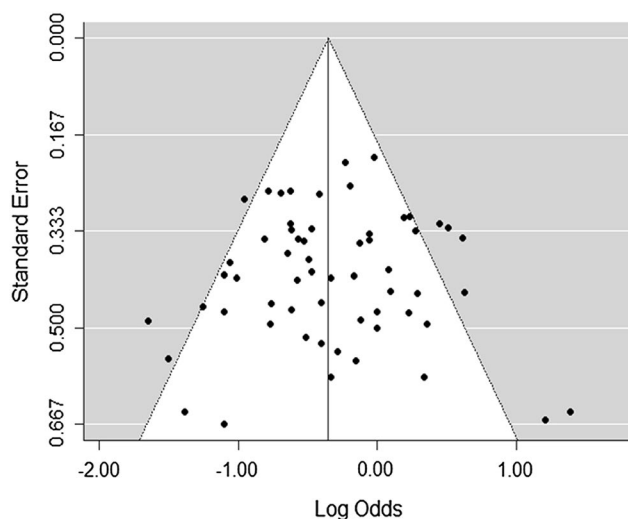
Fig. 3 Funnel plot of total included studies reporting 1 year overall survival
