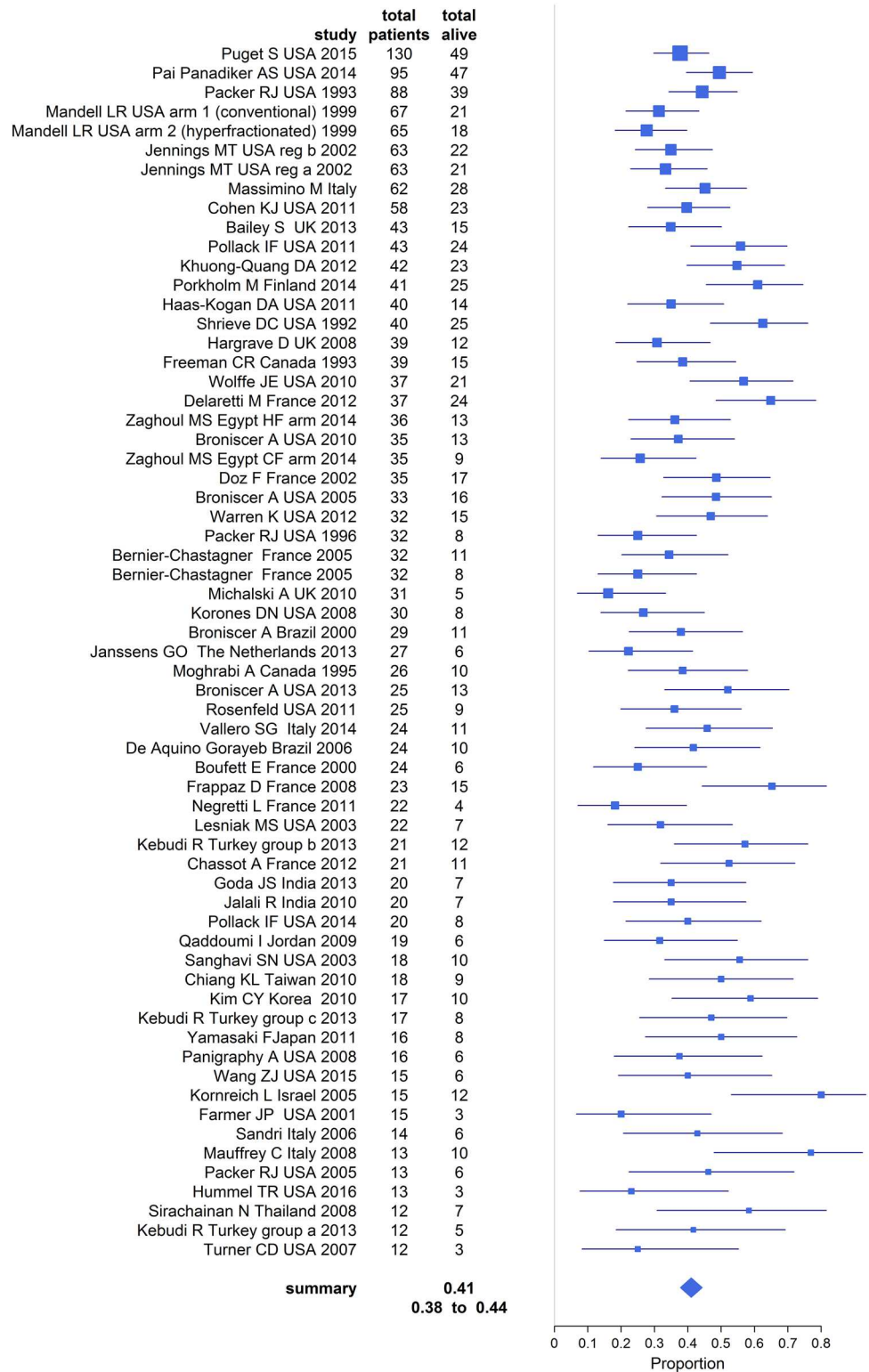
Fig. 2 Pooled estimate of overall survival at 1 year
