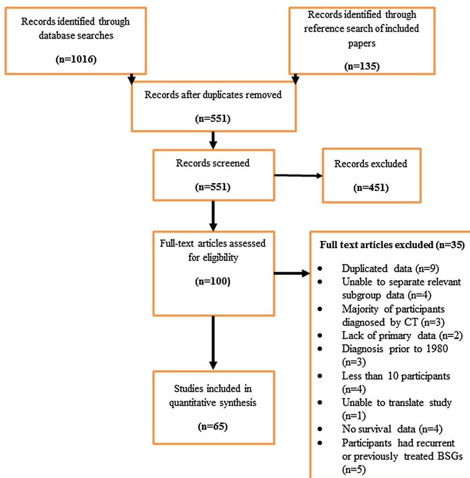
Fig. 1 Summary of the screening process
