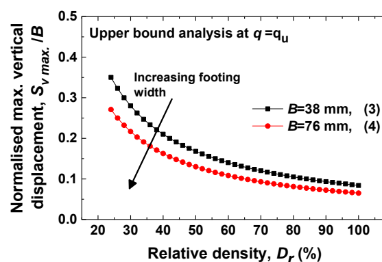
Fig. 6 Variation of normalised maximum vertical displacement in sand under the ultimate load q_u for different cases of footing widths
