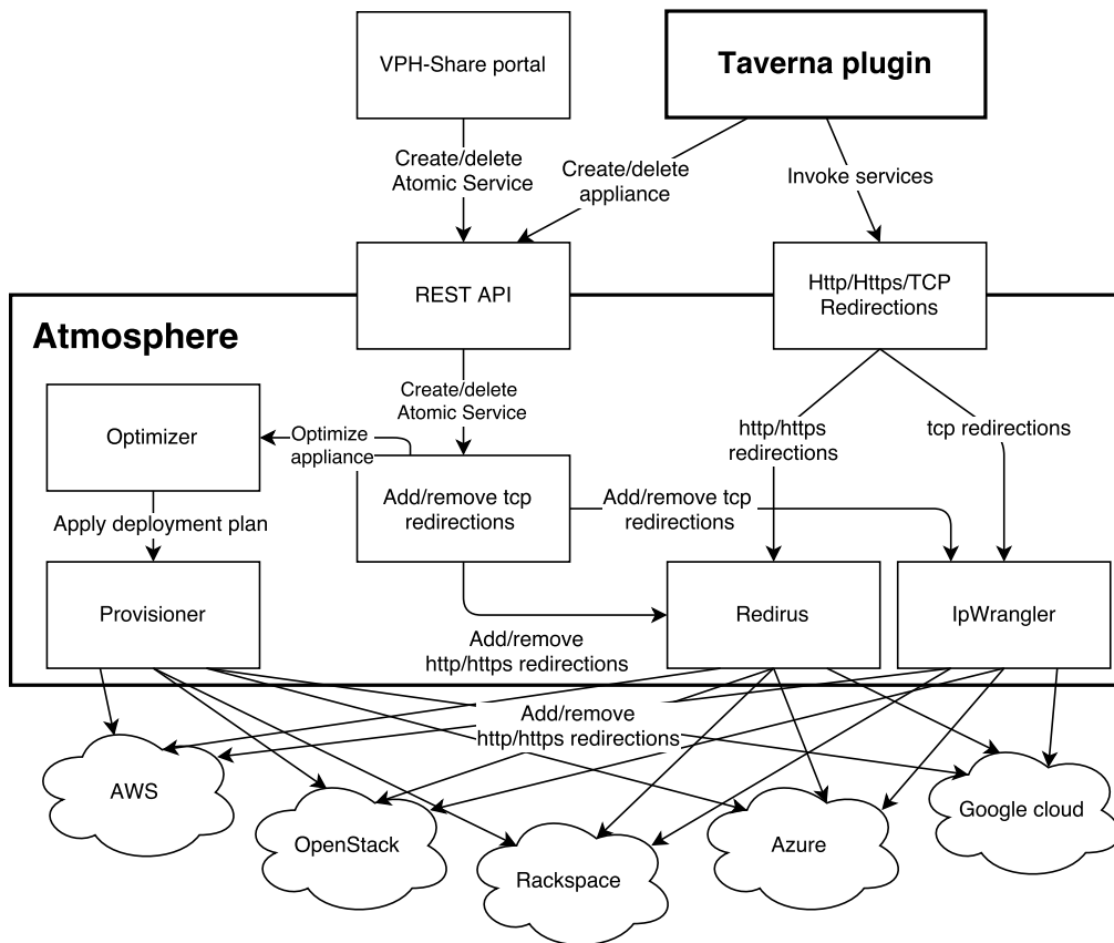
Figure 1: Atmosphere conceals differences between different compute sites and delivers unified REST interfaces used by the Taverna plugin and VPH-Share portal. When a REST request arrives, it is decoded and analysed by the Optimiser component whose main role is to prepare an optimised virtual machine deployment plan for every required Atomic Service. Subsequently, the plan is implemented by the provisioner (which starts/stops/reconfigures virtual machines). Once the required virtual machines are running, access is configured by two components: Redis, which manages HTTP/HTTPS redirections, and IPWrangler, responsible for TCP redirection management.
