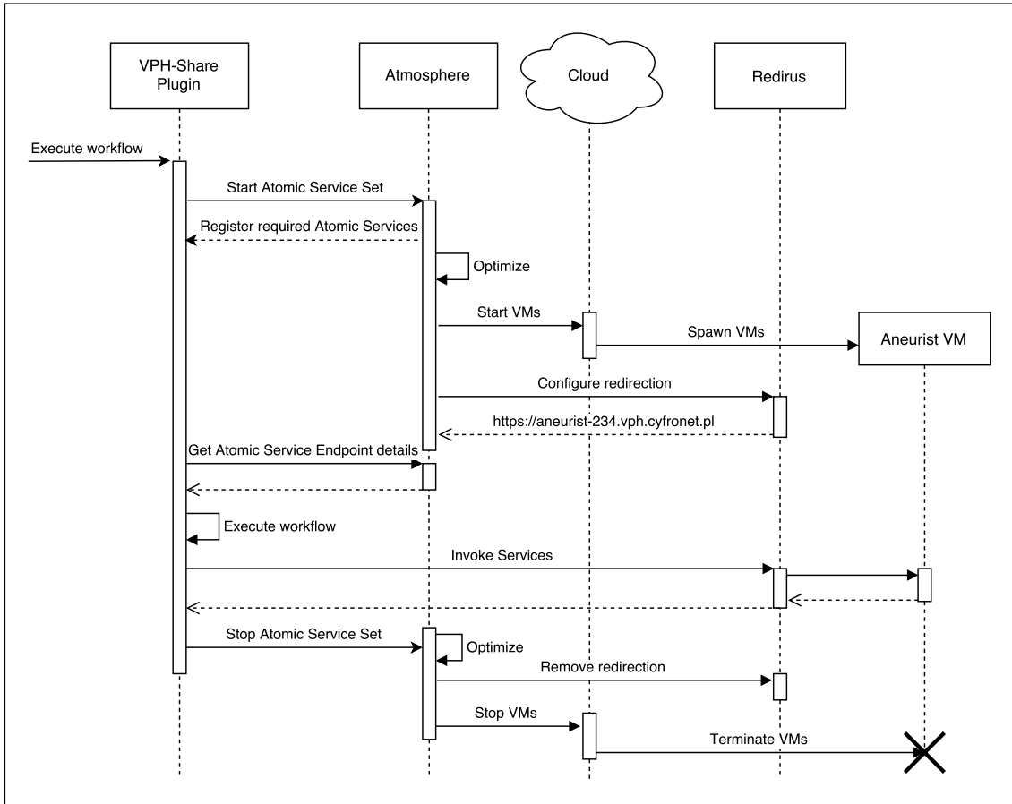
Figure 2: Taverna - Atmosphere interactions in the workflow execution phase. Workflow execution involves optimisation, spawning VM(s) with the required services installed, setting up redirections, execution of the workflow and - finally - freeing up resources used by the workflow.
