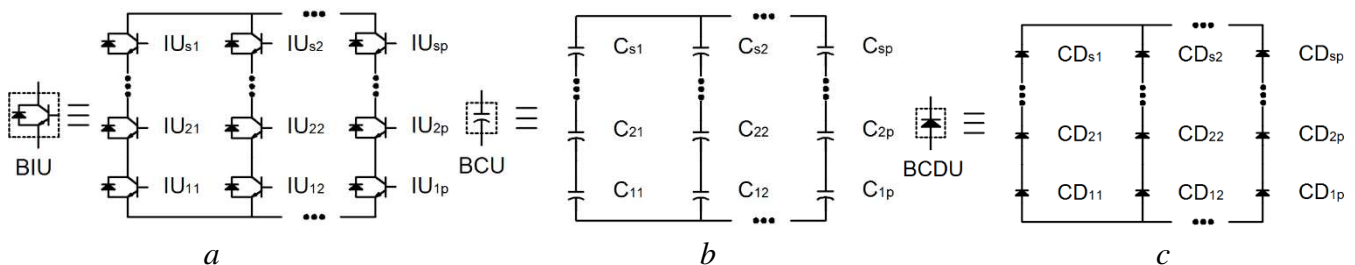
Fig. 2 Representation of a a Basic IGBT Unit (BIU)
