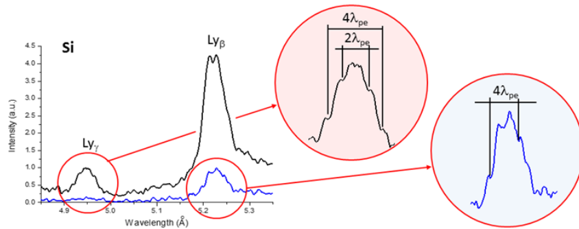
Figure 2. Observation of the Langmuir dips in Ly \beta (blue trace) and Ly \gamma (black trace) corresponding to different incident laser irradianations 0.24 \cdot 10^{21} \text{ Wcm}^{-2} (blue trace) and 1.01 \cdot 10^{21} \text{ Wcm}^{-2} (black trace).
