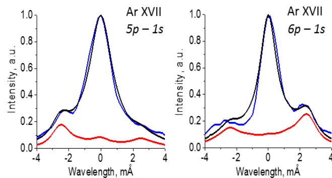
Figure 6. Ar XVII He \delta and \epsilon profiles obtained at J-KAREN at I_L=3 \cdot 10^{18} \text{ Wcm}^{-2} . The blue lines are for the experimental profiles, the solid red lines for the theoretical profiles from a bi-chromatic region and the solid black lines for the total theoretical profiles including a region of no-periodic-field. The black lines exhibit satellites at 2\omega_L .
