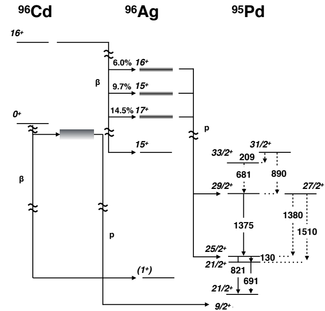
Figure 3: Proposed decay scheme for the \beta decay and \beta p decay of the 16^+ isomer in ^{96}\text{Cd} , the transitions marked with dashed lines were not observed but are within the available angular momentum of the proton decay. The calculated branching ratios to the GT resonance states in ^{96}\text{Ag} , extracted from LSSM calculations, are also presented. The partial decay scheme of ^{95}\text{Pd} was taken from [11]
