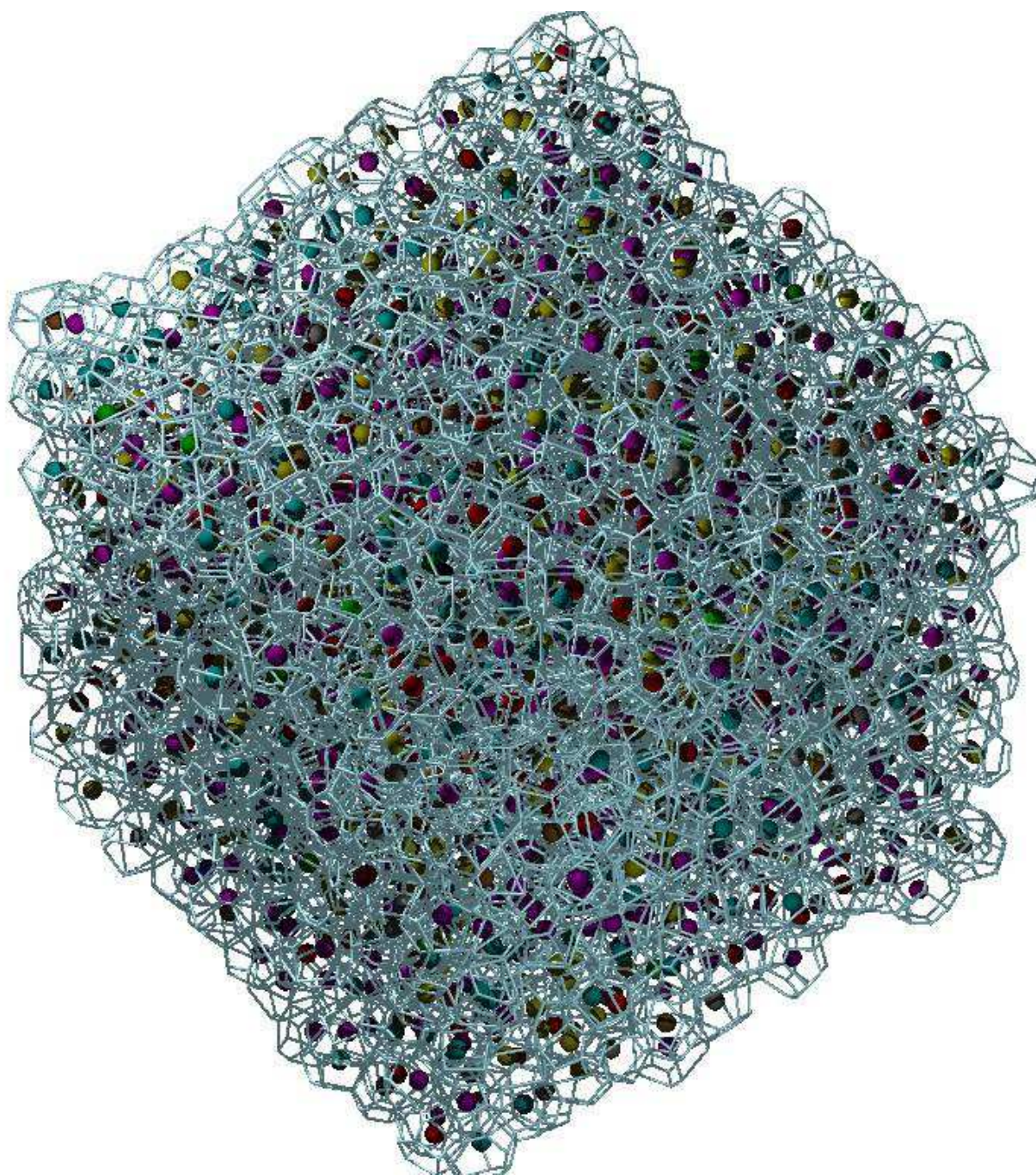
Fig. 5 A snapshot of the final configuration for \text{Mg}_{90}\text{Zn}_{15}\text{Ca}_5 glass with calculated Voronoi polyhedra. Mg, Zn and Ca atoms are represented with the spheres coloured with respect to different coordination numbers.
