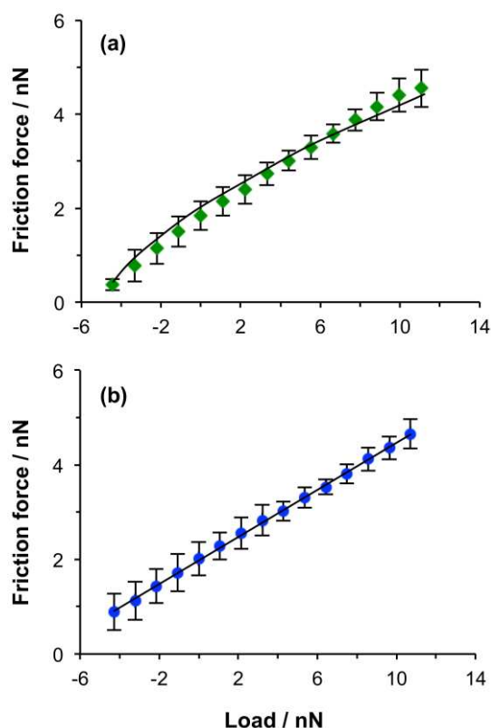
Figure 3. Friction-load plots obtained for PCysMA brushes with a dry thickness of 7 nm immersed in (a) water and (b) ethanol. Data acquired in the former solvent have been fitted using the DMT model, while a straight line has been fitted by linear regression for the data set acquired in the latter solvent.
