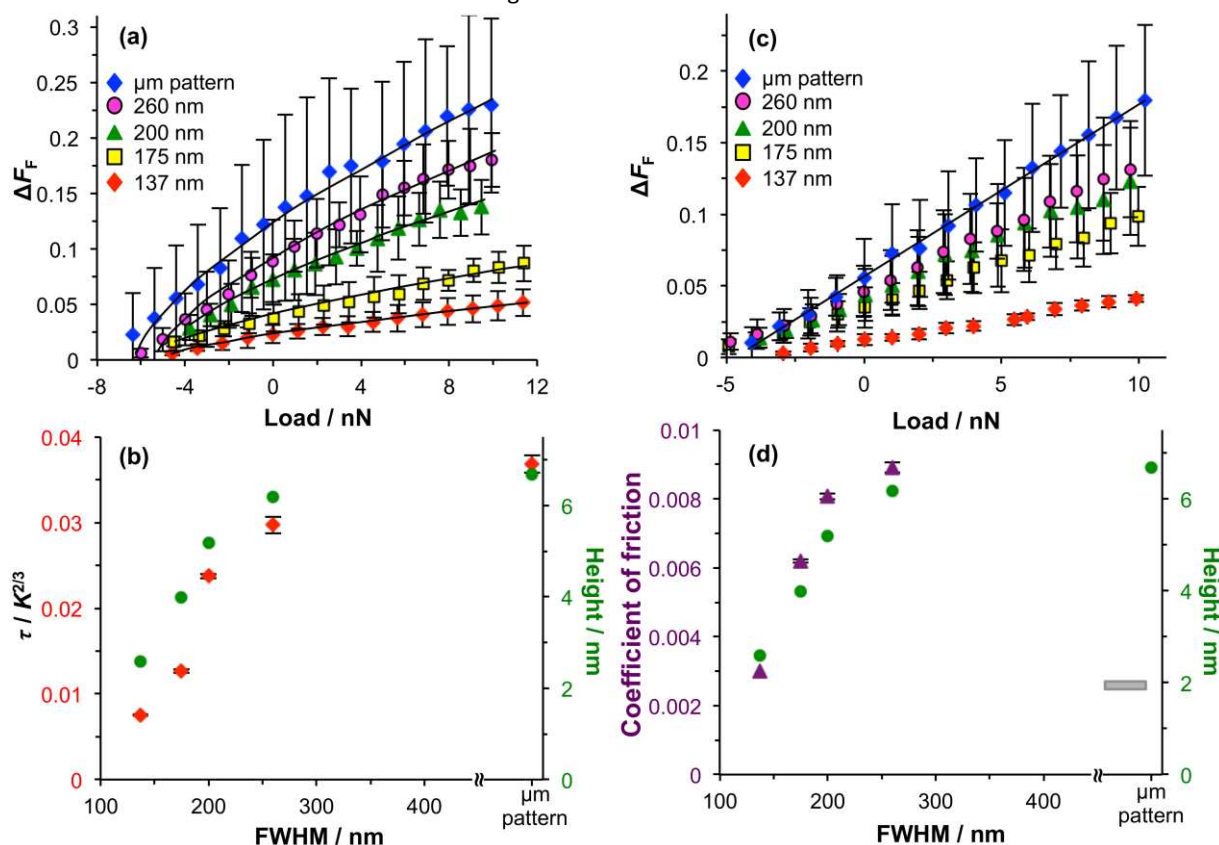
Figure 6. (a) Variation in the peak-trough friction difference with load for brushes of varying (dry) feature size after immersion in water. Data fits (black lines) were obtained assuming DMT mechanics. (b) Variation in the surface shear strength with feature size for brushes immersed in water (diamonds). (c) Variation in the peak-trough friction difference with load for brushes of varying feature size immersed in ethanol. (d) Variation in the coefficient of friction with dry feature size for brushes immersed in ethanol (triangles). (c) and (d) also show the variation in heights of the dry polymer structures as a function of dry feature size.
