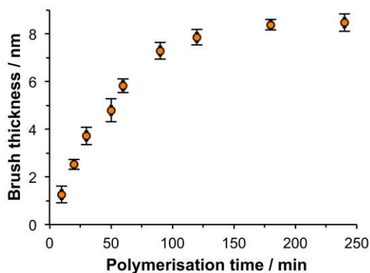
Figure 1. Variation in dry brush thickness with polymerisation time for PCysMA brushes as determined using ellipsometry. Micropatterned Brushes
