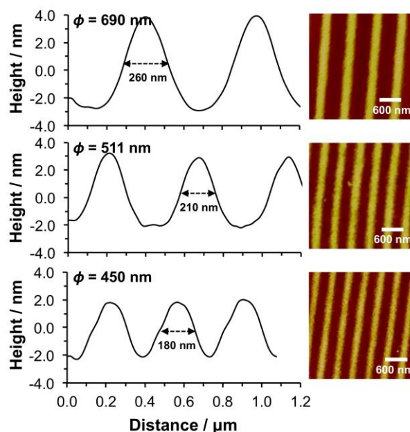
Figure 5. Left: mean AFM height sections through topographical images (right) acquired for nanostructured PCysMA brushes formed with periods \phi in the range 450 - 690 nm.
