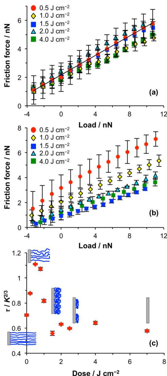
Figure 4. (a) Friction-load plots acquired in ethanol for a series of PCysMA brushes grown from bromine-functionalised planar surfaces subjected to varying UV doses. The data were fitted using linear regression and linear friction-load relationships were observed in all cases. For clarity, only one fit is shown (for a UV dose of 0.5 \text{ J cm}^{-2} ). (b) Friction-load plots acquired in water for a series of PCysMA brushes grown from bromine-functionalised surfaces subjected to varying UV doses. Fits are shown for UV doses of 0.5 \text{ J cm}^{-2} (DMT) and 2.0 \text{ J cm}^{-2} (linear). (c) Variation in the surface shear strength determined in water as a function of the UV dose. Schematic diagrams illustrate the change in polymer conformation with grafting density.
