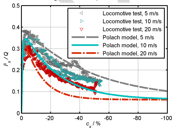
Fig. 11: Variation of adhesion calculated with the Polach model and comparison with locomotive test data in dry condition. The Polach parameters from the curve at 10 m/s have been used for calculating the Polach adhesion curves at 5 m/s and 20 m/s (with deactivated linear regression models).
