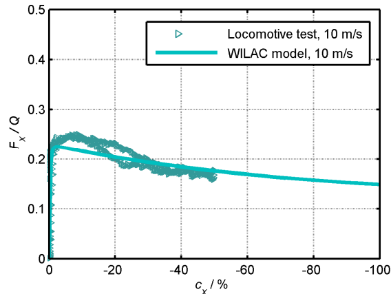
Fig. 10: Comparison of WILAC model results with locomotive test data from literature [Six2015] in wet surface condition.
