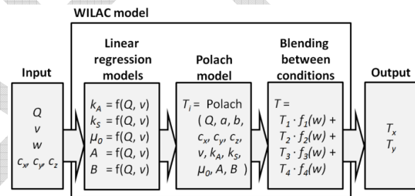
Fig. 4: General structure of the WILAC model for calculating creep forces in dry, moist and wet conditions.
