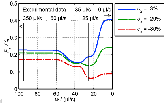
Fig. 8: Change of adhesion F_x/Q as a function of water flow rate w for different fixed values of longitudinal creep c_x . Water flow rates w where experimental data have been recorded are marked by vertical lines.
