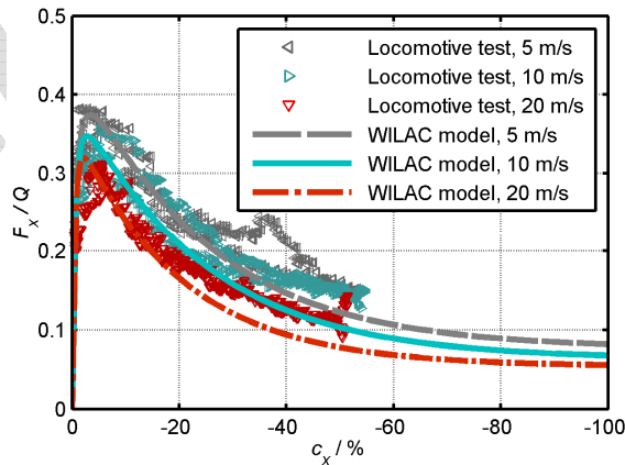
Fig. 9: Comparison of WILAC model results with locomotive test data from literature [Six 2015] in dry surface condition.
