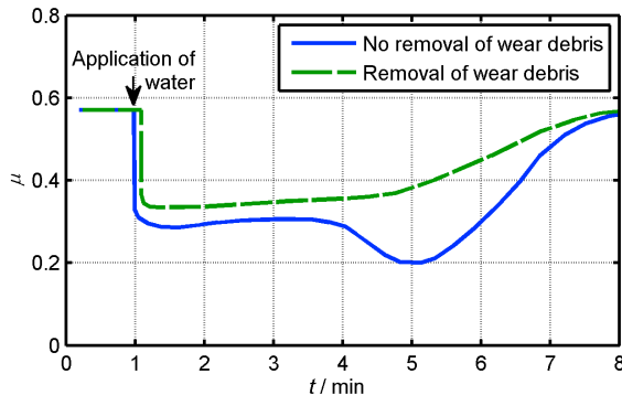
Fig. 1: Schematic change of adhesion in an Amsler experiment when the surface dries up after an initial application of water; Solid line: Adhesion minimum without continuous removal of wear debris; Dashed line: Continuous removal of wear debris by wire-brushing the surface; data reproduced from [Beagley 1975].
