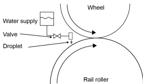
Fig. 2: Drop-wise application of low amounts of water by a gravity fed water application system.
