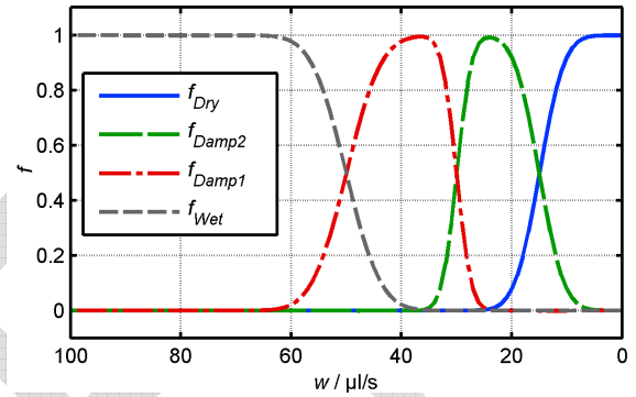
Fig. 5: Weights f_i as a function of the water flow rate w , which are used to calculate the actual adhesion T_i/Q .
