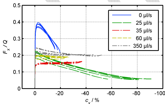
Fig. 3: Measured adhesion in the tram wheel test rig experiments as a function of the water rate at 4.2 kN normal force and 5 m/s rolling speed.
