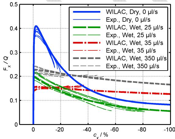
Fig. 7: Experimental data (thin lines) used for model parameterisation and associated WILAC model results (thick lines) for different water flow rates w at 4.2 kN normal force and 5 m/s rolling speed.
