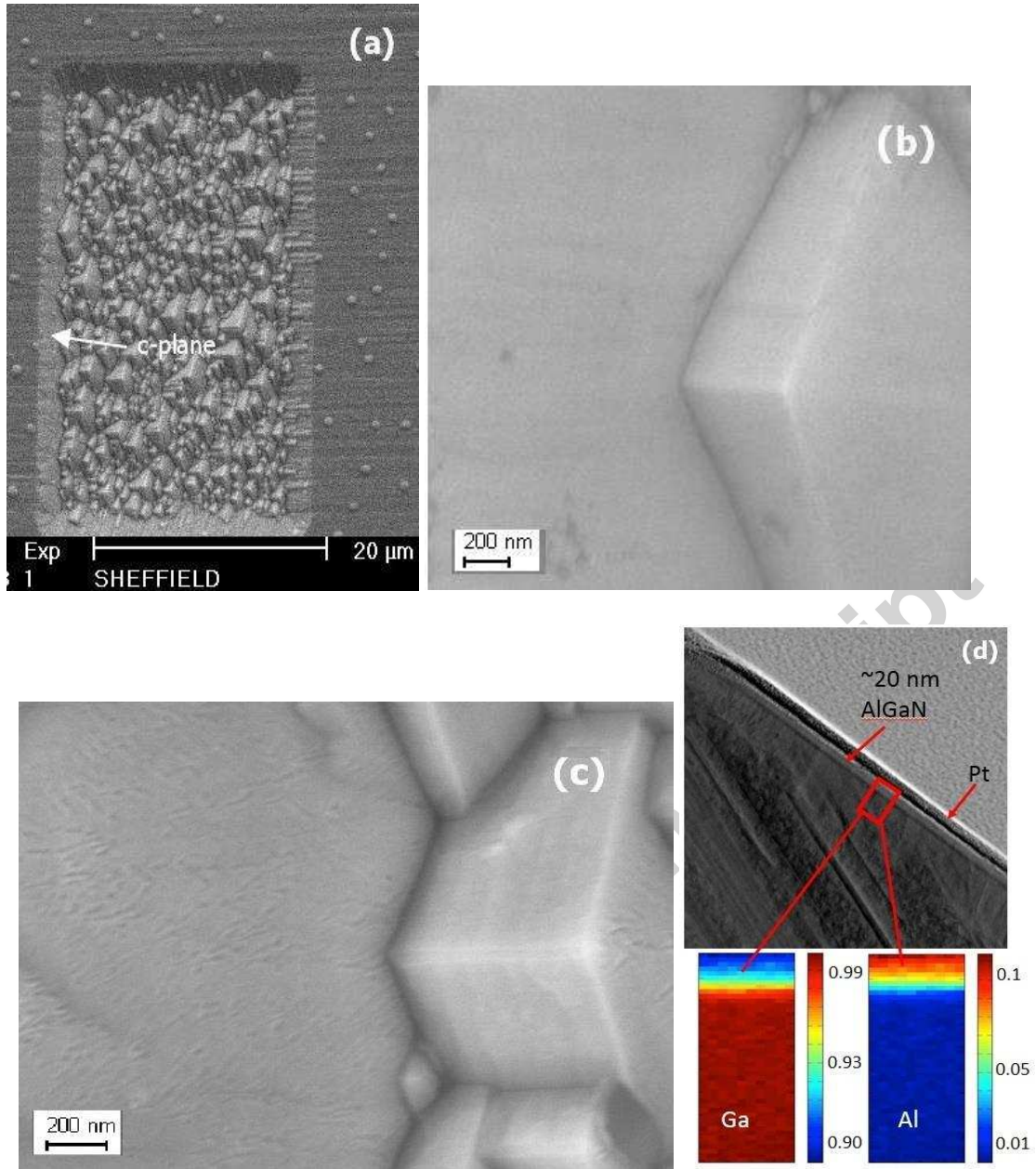
Fig. 3. (a) The SEM images of etched (11-22) GaN after MBE regrowth under Ga-rich conditions. The high resolution SEM image of the c-plane sidewall (b) before regrowth, and (c) after regrowth. (d) The cross-sectional TEM image of the regrown c-plane side wall with EDS mapping
