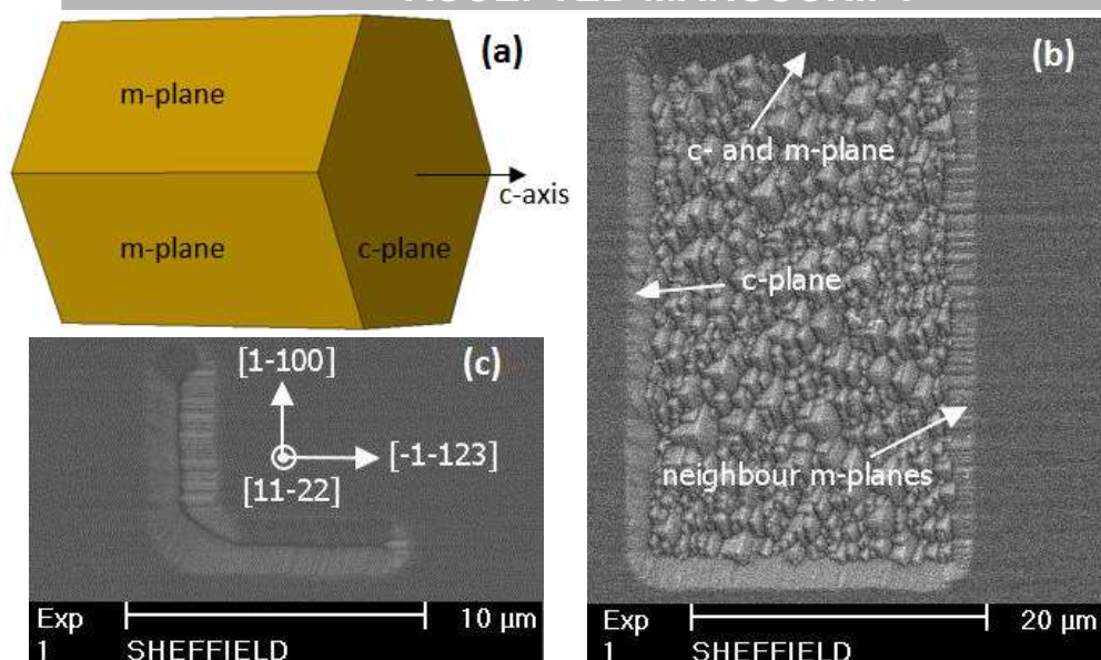
Fig. 2. (a) The schematic structure of a unit cell of wurtzite GaN oriented in [11-22] direction showing the crystallographic planes of the facets. The SEM images of the etched sample in the (b) 22\ \mu\text{m} opening region and (c) 2\ \mu\text{m} opening region.
