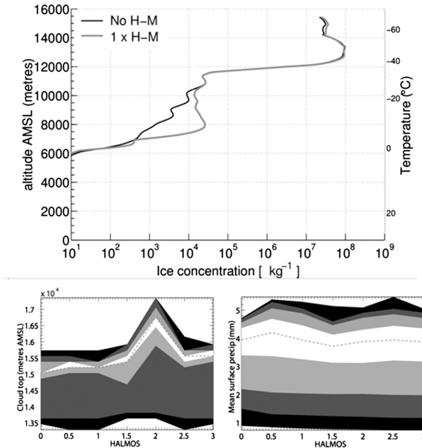
FIG. 7-9. Modeling examples using the Weather Research and Forecasting model showing the impact of SIP on cloud evolution. (top) After Connolly et al. (2006b) , the impact of a rime-splintering (H-M) parameterization on ice crystal number mixing ratio. (bottom left) Cloud-top height as a function of H-M (here labeled “HALMOS”) splinter production efficiency (1.0 = 1 times standard H-M rate). Shaded contours represent percentiles [gray shadings: 10%–40% and 60%–90% (at 10% intervals)] of domain. (bottom right) Domain mean surface precipitation as a function of H-M splinter production efficiency (from Connolly et al. 2006a ).
