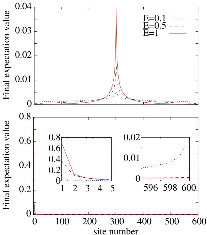
Fig. 3. Steady state site occupation probabilities versus site number i , shown for three selected disorder strengths E = 0.1 (dotted line), E = 0.5 (dashed line), and E = 1.0 (solid line), for a chain of length N = 600 , when the excitation is injected at site i = 1 (bottom panel) and i = \frac{N}{2} (top panel). The insets in the bottom panel focus on the initial (left inset) and final (right inset) sites of the chain.
