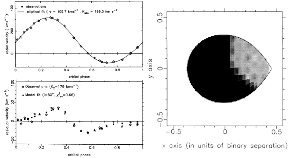
Fig. 4. Radial-velocity curve fitting of the polar AM Her. Upper-left: Radial-velocity curve of the NaI absorption doublet around 8190\text{\AA} [9]. Lower-left: Residual-velocity curve, i.e. the motion of the centre-of-mass of the secondary has been removed [10]. Right: Surface map of AM Her – the light region is where the NaI doublet is weakest [10].
