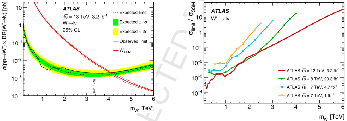
Fig. 3. Median expected (dashed black line) and observed (solid black line) 95% CL upper limits on cross-section times branching ratio ( \sigma \times B ) in the combined channel, along with predicted \sigma \times B for W'_{SSM} production (red line). Uncertainties in \sigma \times B from the PDF, \alpha_s and scale are shown as a red-dashed line. The bands for 68% (green) and 95% (yellow) confidence intervals are also shown. The vertical dashed line indicates the mass limit of the 8 TeV data analysis [2]. (For interpretation of the references to colour in this figure legend, the reader is referred to the web version of this article.)
