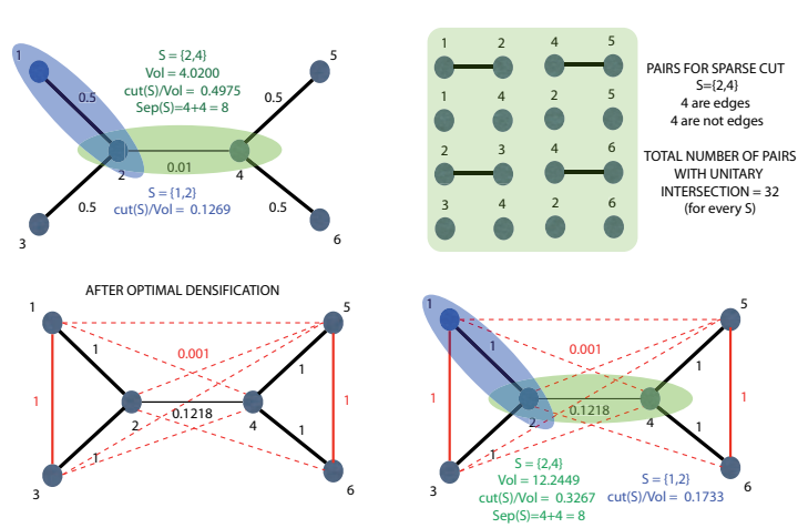
Fig. 1. Densification example. Graph G with n = 6 nodes. Top-left: Cuts associated with a couple of sets S = \{2, 4\} and S = \{1, 2\} . We define \text{Sep}(S) = \sum_{u,v} \delta_S(u, v) . For the cut S = \{2, 4\} there are 4 pairs associated with edges and 4 pairs not associated with edges (top-right). This means that this cut is sparse since \frac{\text{cut}(S)}{\text{Vol}(G)\text{Sep}(S)} = 0.0622 . In bottom-left we show the densification H result solving the spectral version of problem P1 (Eq. 2) through the dual problem P2 (Eq. 6) for C = 2 . Red-dotted lines have weight 0.001. Some cuts have lower values, for instance the one for S = \{2, 4\} , whereas others such as the cut for S = \{1, 2\} increase (bottom-right). This is important since the new volume has also increased. All cuts satisfy \frac{\text{cut}_H(S)}{m(H)} \leq C \cdot \frac{\text{cut}_G(S)}{m(G)} .
