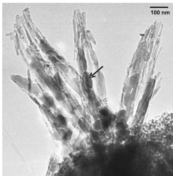
Figure 6 BF TEM micrograph of a nanostructure emerging from the alumina support
