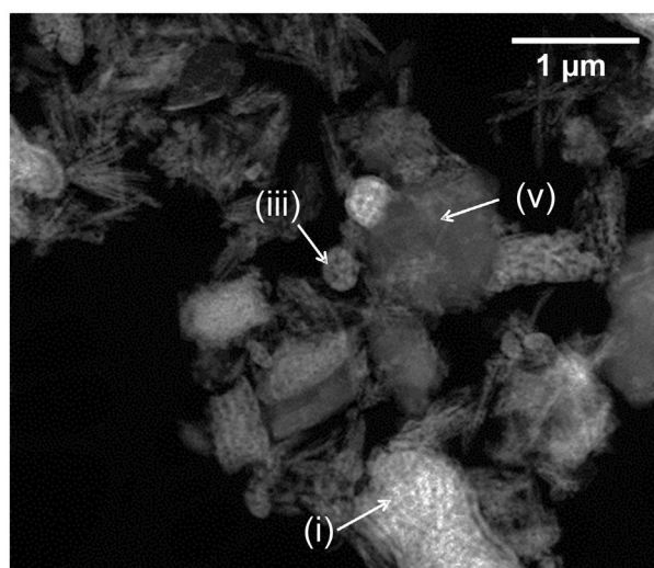
Figure 5 Low magnification HAADF STEM micrograph of post reaction sample: (i) highly porous particles of size 500 nm–2 \mu\text{m} ; (iii) rounded crystalline particles of size \sim 50 –100 nm; (v) pure \text{Al}_2\text{O}_3 .
