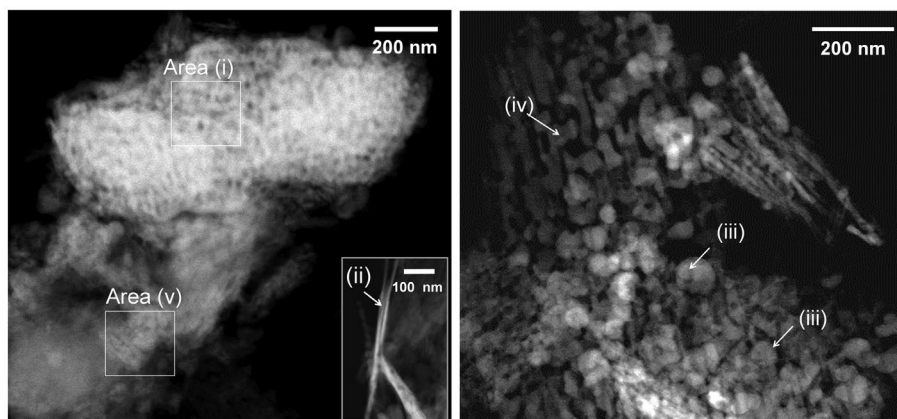
Figure 4 HAADF STEM micrographs of fresh catalyst showing the different microstructures found: areas (i)–(iv) contain both Fe and Al and are defined as (i) highly porous particles of size 500 nm–2 \mu\text{m} ; (ii) crystalline “rods” of \sim 500 nm length; (iii) rounded crystalline particles of size \sim 50 –100 nm; (iv) plate-like structures; while Area (v) consists of pure \text{Al}_2\text{O}_3 . Note: Analysis of areas (i)–(v) is presented in Table 2.
