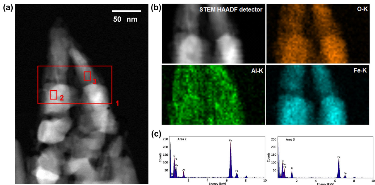
Figure 7 a HAADF STEM image of one of the needle like structures found in the post-reaction catalyst; b EDS mapping of Area 1 indicated in a; c EDS spectra from Areas 2 and 3 indicated in a
