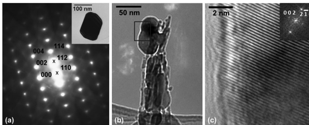
Figure 8 a Diffraction pattern recorded parallel to the [1\bar{1}0] zone axis corresponding to the \epsilon\text{-Fe}_2\text{C} isolated particle shown in the inset; b BFTEM micrograph of an elongated alumina structure containing crystalline particles; c HR image of the highlighted area in b: the strong fringes correspond to the (2\bar{1}0) plane
