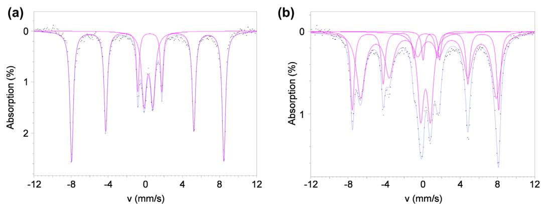
Figure 2 Fitted ^{57}\text{Fe} Mössbauer spectra: a fresh catalyst, and b catalyst post-reaction
