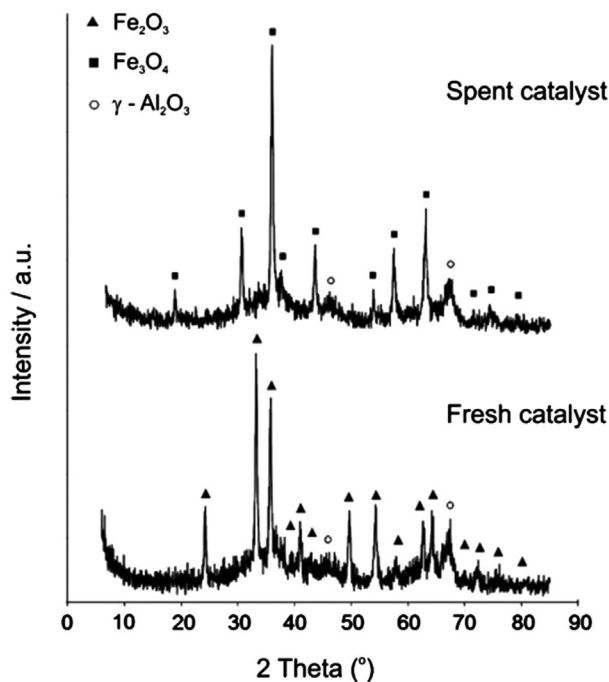
Figure 1 X-ray diffraction patterns of fresh and spent catalysts
