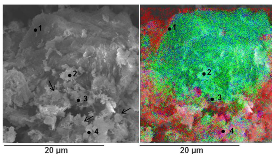
Figure 3 Low magnification (3500 \times ) SEM a and EDS map b of the fresh FeO x /γ-Al 2 O 3 catalyst showing the distribution of iron (red), oxygen (blue) and aluminum (green) elements
