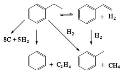
Scheme 1 Reaction scheme for ethylbenzene dehydrogenation 11
