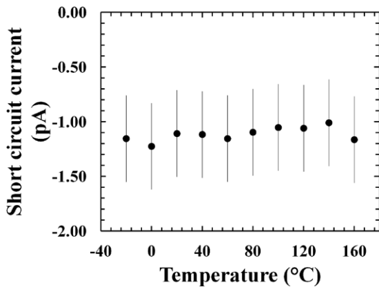
Figure 7. Short circuit current as a function of temperature for a single cell of the \text{Al}_{0.52}\text{In}_{0.48}\text{P}^{55}\text{Fe} radioisotope microbattery; in particular, results from D1 under illumination of the ^{55}\text{Fe} x-ray source are shown.
