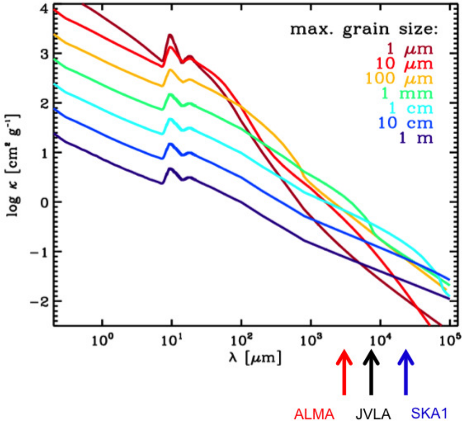
Figure 1: Opacity curves for grains of different sizes showing the flattening of the slope at cm wavelengths as the grains become cm-sized. The wavelengths at which ALMA, JVLA and SKA1-MID can deliver matching-beam data with a resolution of 40 mas are indicated. This corresponds to the \sim 4 au radius of the snow line in the nearest proto-planetary disks.
