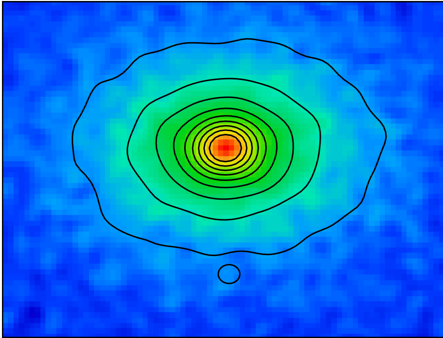
Figure 2: Simulated continuum image of a proto-planetary disk using a 2 \times 2.5 GHz bandwidth from 8.8 to 13.8 GHz. Contours run from 5, 10, 15, ..., 45 times the 0.07 \mu\text{Jy}/\text{beam} noise level. The image is about 0.85 \times 0.65 arcseconds in size and the 35 \times 40 mas beam is indicated. See text for details. Note that real disks are likely to have significant structure in them as in Figure 1 of Testi et al. (2015).
