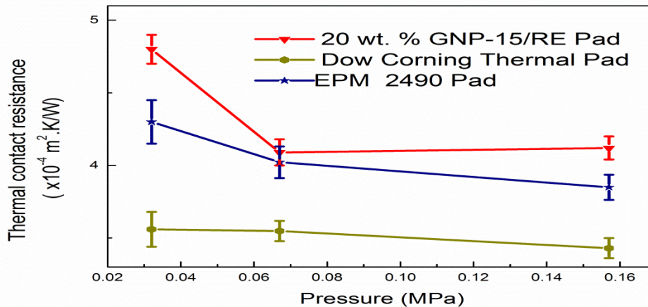
Fig. 2. Thermal contact resistance vs. applied pressure of GNP/rubbery epoxy and commercial pads measured at ~40 °C between smooth copper cylinders.
