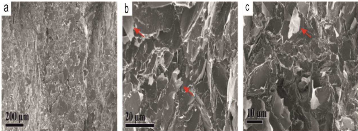
Fig. 1. SEM images of GNP-15/RE composite produced by roll mill at loading of (a & b) 25 wt.% and (c) 25 wt.% GNP-5/RE composite, arrows point towards GNPs in the matrix.
