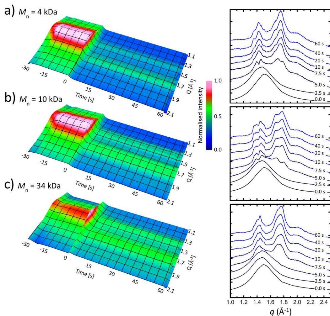
Figure 7: In situ grazing incidence scattering data showing the development of crystallinity for PEO ( M_n = 4 kDa, 10 kDa and 34 kDa) spuncast from 10 wt% THF solutions at 1,500 rpm. a-c) Radially integrated scattering data as a function of time with corresponding cross sections at between 0 and 60 s, for 4 kDa (a), 10 kDa (b) and 34 kDa (c) PEO.
