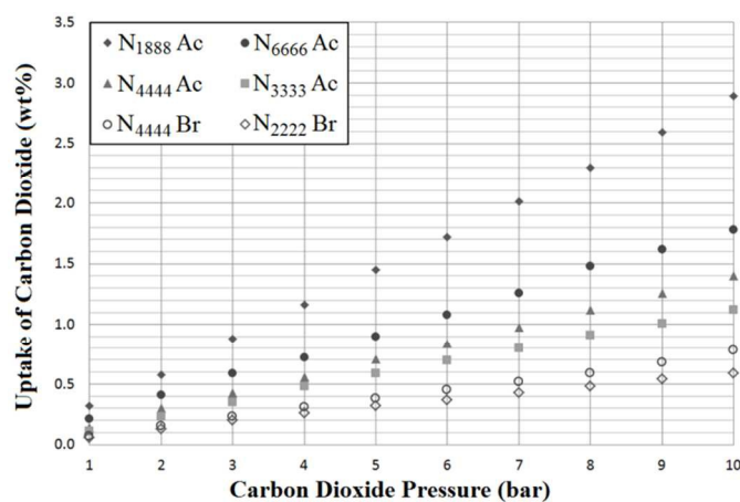
Figure 5: Adsorption of carbon dioxide by selected tetraalkylammonium solid ionic liquids (SoILs) at a pressure range of 1-10 bar, 298 K. Uptake is given as mass CO 2 adsorbed per gram of sorbent.
