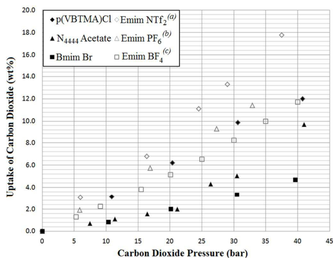
Figure 8: Results of higher pressure testing of selected ionic liquids from this work (solid markers) compared with literature results for common RTILs used for CO_2 adsorption at 298 K (hollow markers). (a) Zhu 25 , (b) Peters 26 , (c) Lee 27 Uptake is given as mass CO_2 adsorbed per gram of sorbent.
