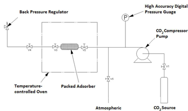
Figure 3: Process flow diagram of high pressure testing apparatus
