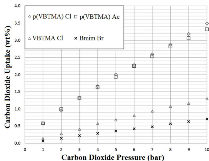
Figure 6: Adsorption of carbon dioxide by selected polymer and solid ionic liquids at a pressure range of 1-10 bar, 298 K. Uptake is given as mass CO 2 adsorbed per gram of sorbent.
