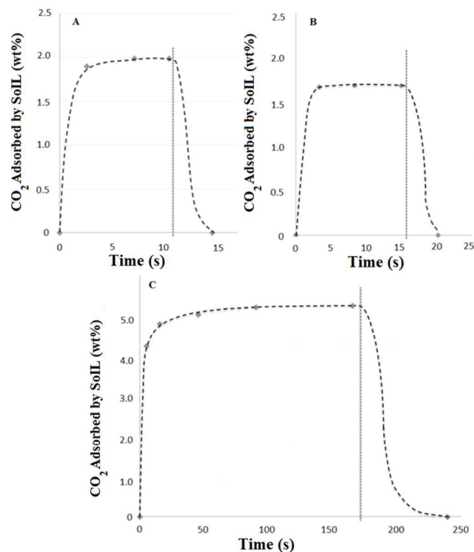
Figure 9: Adsorption and desorption profiles of selected SoILs at 15 bar. Dashed trendline showing approximate CO 2 uptake curve for clarity. Vertical grey line indicates initiation of depressurisation. (A) N 4444 Acetate. (B) BMim Bromide. (C) p(VBTMA) Chloride.
