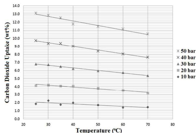
Figure 10: The effect of temperature on the CO 2 uptake capacity of N 4444 Acetate at different pressures
