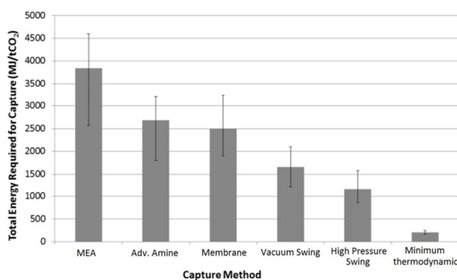
Figure 1: Comparison of calculated energy costs of different CO 2 capture methods, MEA 16 , Advanced Amine 17 , Membrane 18 , Vacuum Swing 19 , High Pressure Swing was calculated from preliminary process model [see main text] and was found to be in agreement with literature values 20 . Minimum thermodynamic separation costs were calculated from entropy of de-mixing.
